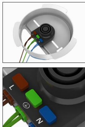
I Internal wiring details
